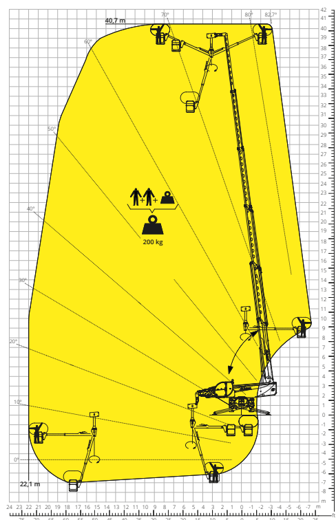
Load chart with OVER-UNDER PLATFORM - NEGATIVE ATT - 01 - 024
