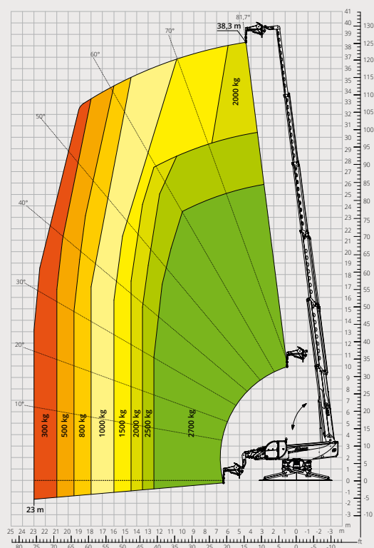
Load chart with JIB WITH WINCH, 2,700 kg ATT - 04 - 017
